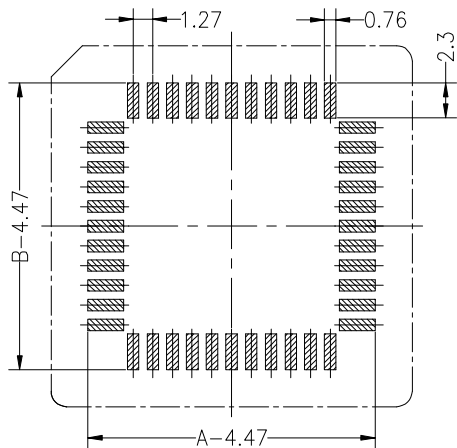
PCB LAYOUT
