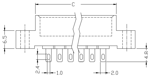
SOLDER TYPE (P/N: CKSL-XXS)
