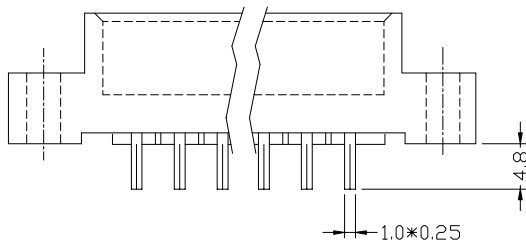
DIP TYPE (P/N: CKSL-XXD)
