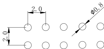
P. C. B Hole Layout
