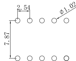
Recommended P.C. Board Hole Layout
